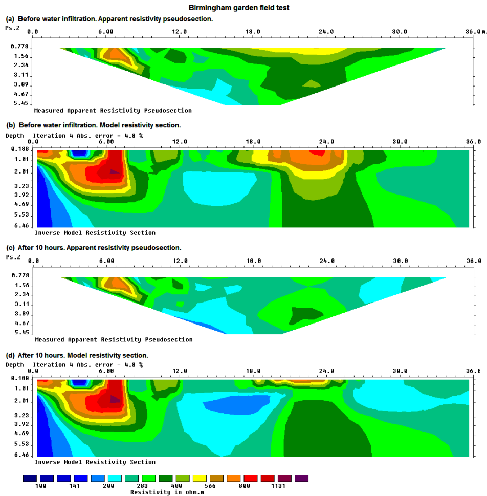
Figure 40. Apparent resistivity and inversion model sections from the Birmingham time-lapse experiment. (a) The apparent resistivity and (b) inversion model sections from the survey conducted at the beginning of the Birmingham infiltration study. The data and model after 10 hours of irrigation are shown in (c) and (d).
