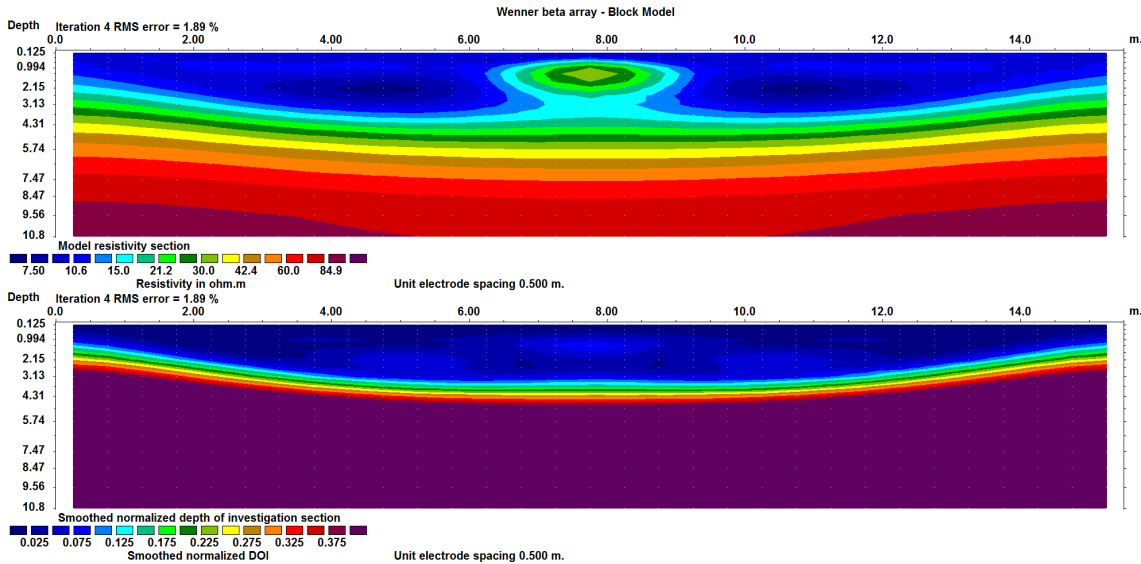
Figure 51. Example DOI plot for the beta.dat file.
