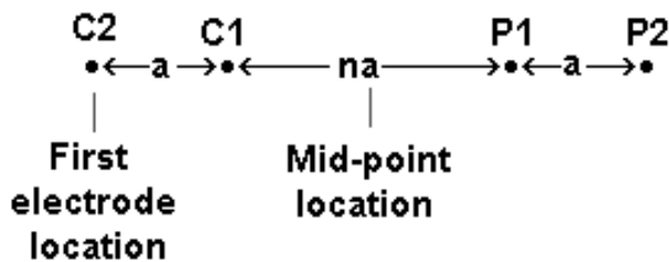
Figure 3. Parameters that specify the location and length of an array in the index based data format.
