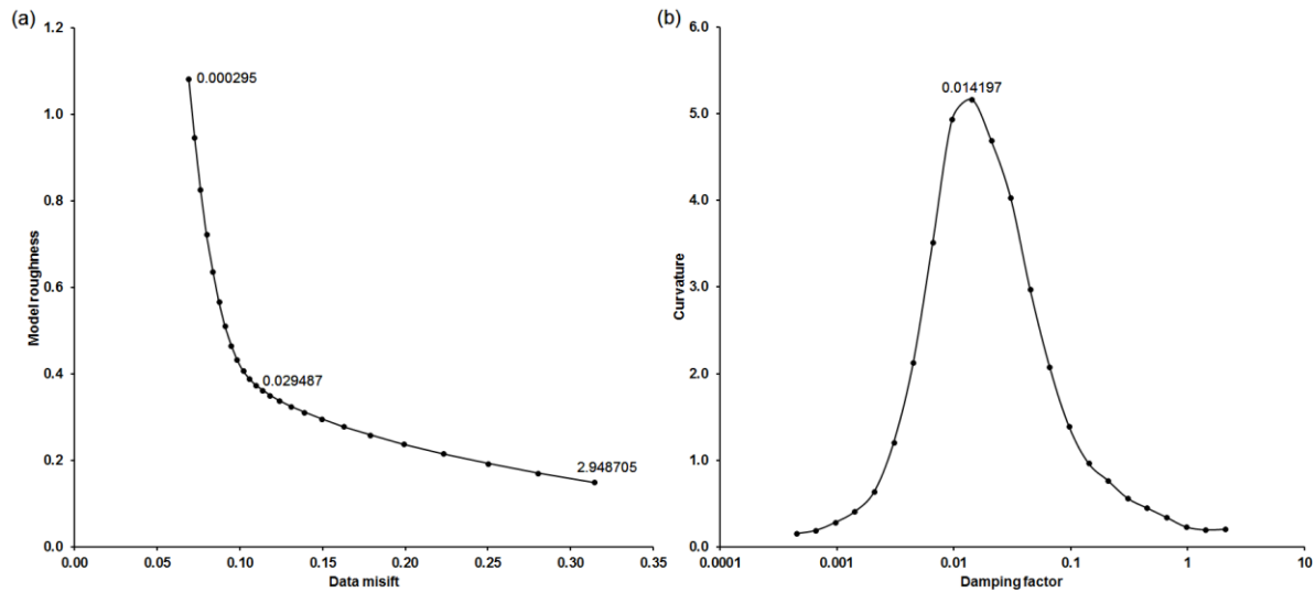
Figure 23. Example L-curve plot to determine the optimum damping factor for the BLUERIDGE.DAT data set. (a) Variation of model roughness with data misfit for a range of spatial damping factor values (a few values are shown near the corresponding points), (b) variation of the curvature of the L-curve with the damping factor.
