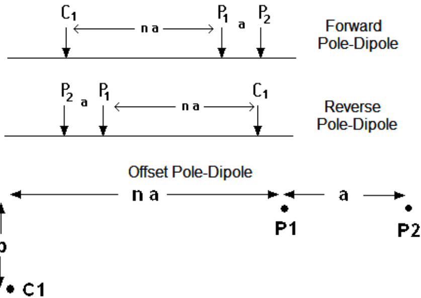
Figure 45. Normal, reverse and offset pole-dipole array arrangements.
