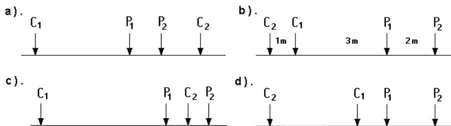
Figure 7. Some possible non-conventional arrays. (a) Non-symmetrical four-electrode Wenner-Schlumberger or gradient type of array. (b) Dipole-dipole array with dipoles of unequal size. (c) A possible but probably non-viable electrode configuration. (d) Highly non-symmetrical dipole-dipole array.
