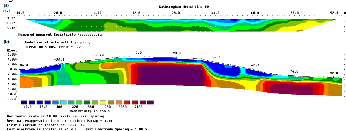
Figure 37. Example of the model for the Rathcroghan Mound data set. (a) Measured apparent resistivity pseudosection. (b) Inverse model section with topography.
