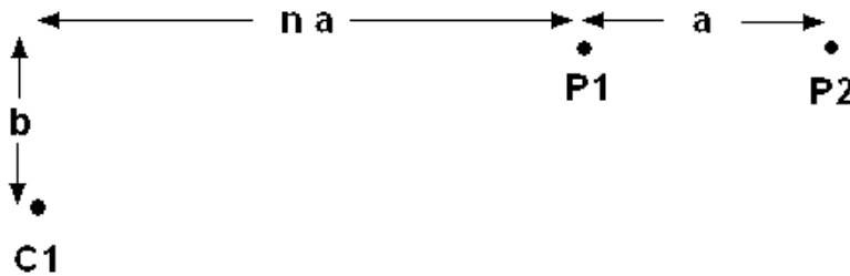
Figure 6. Arrangement of electrodes for the offset pole-dipole array.
