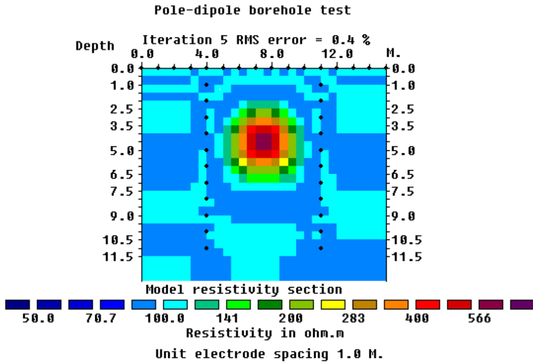
Figure 12. The model obtained after the inversion of the BOREHOLE.DAT data set. The option to use finer blocks with half the size of the spacing between the electrodes was used.
