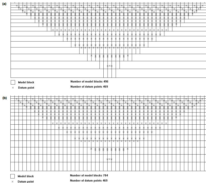
Figure 2. Two possible arrangements of the blocks used in a 2-D model together with the data points in the pseudosection.
