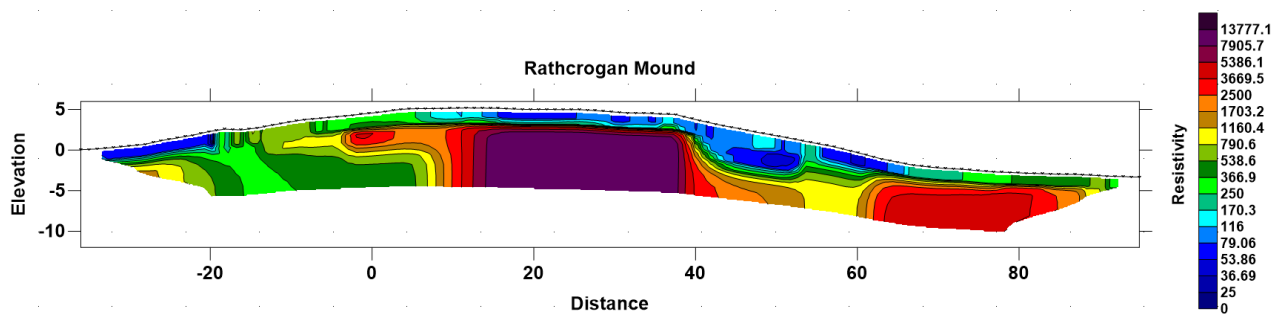
Figure 50. Plot of the RATCHRO.INV file output using Surfer.
