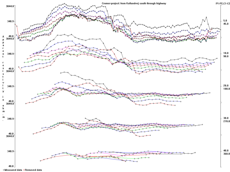
Figure 27. Plot of a CROMER02.DAT multiple gradient array data set in the form of profiles using the approximate pseudodepth method.
