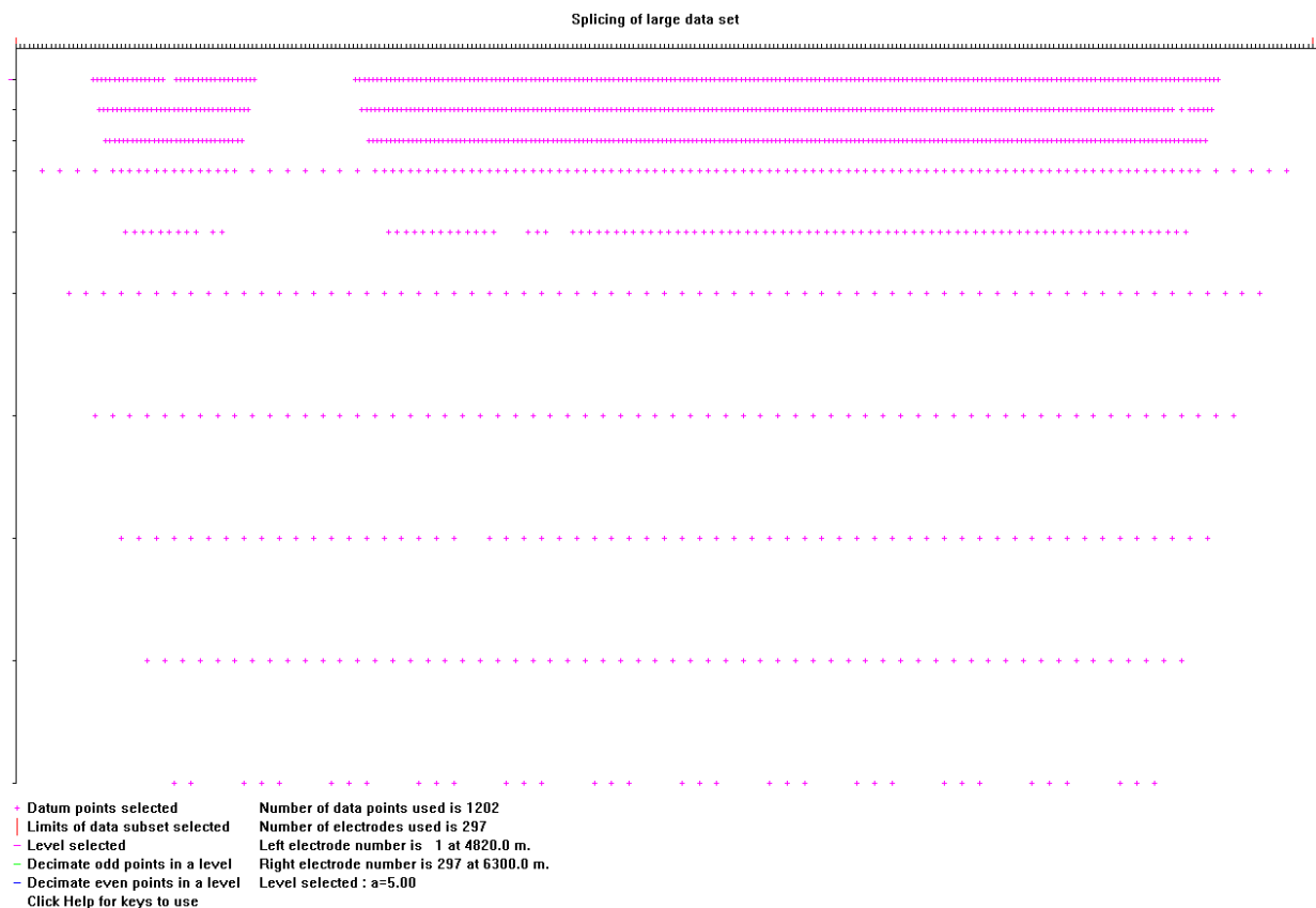
Figure 21. Example of a display using the splice data option for a data set in the indexed base format.
