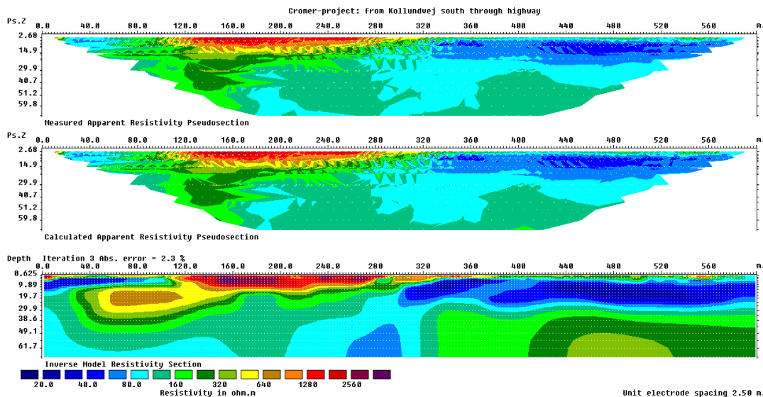
Figure 28. The inversion result of the CROMER02.DAT data set with the apparent resistivity and model sections.
