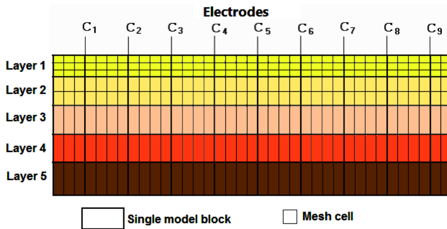
Figure 24. Schematic diagram of mesh and model cells used by forward modeling routine. This example has 4 nodes between adjacent electrodes.
