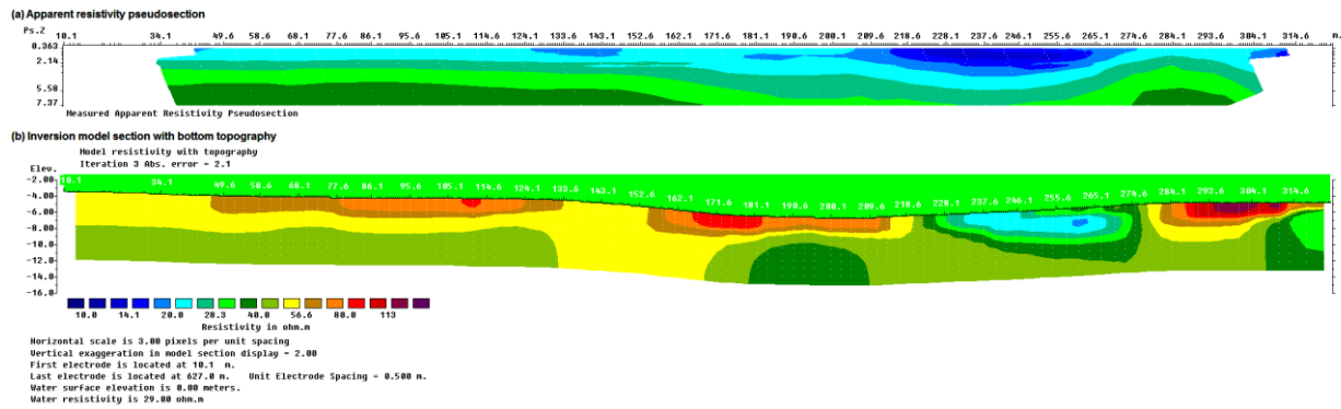
Figure 42. Example of underwater survey. (a) Apparent resistivity pseudosection. (b) Model section with topography. Note the contoured model plot has been extended upwards to the water bottom interface, and the color of the water layer matches the contour scale used for the resistivity sections. This example is from an underwater riverbed survey by Sage Engineering, Belgium.
