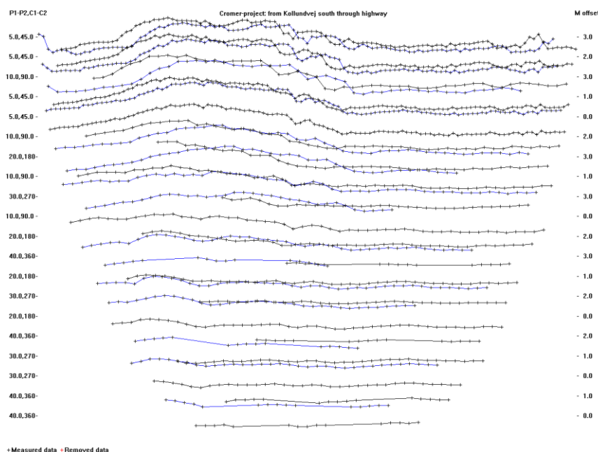
Figure 25. Plot of a multiple gradient array data set in the form of profiles using exact pseudodepths for the CROMER2.DAT file.
