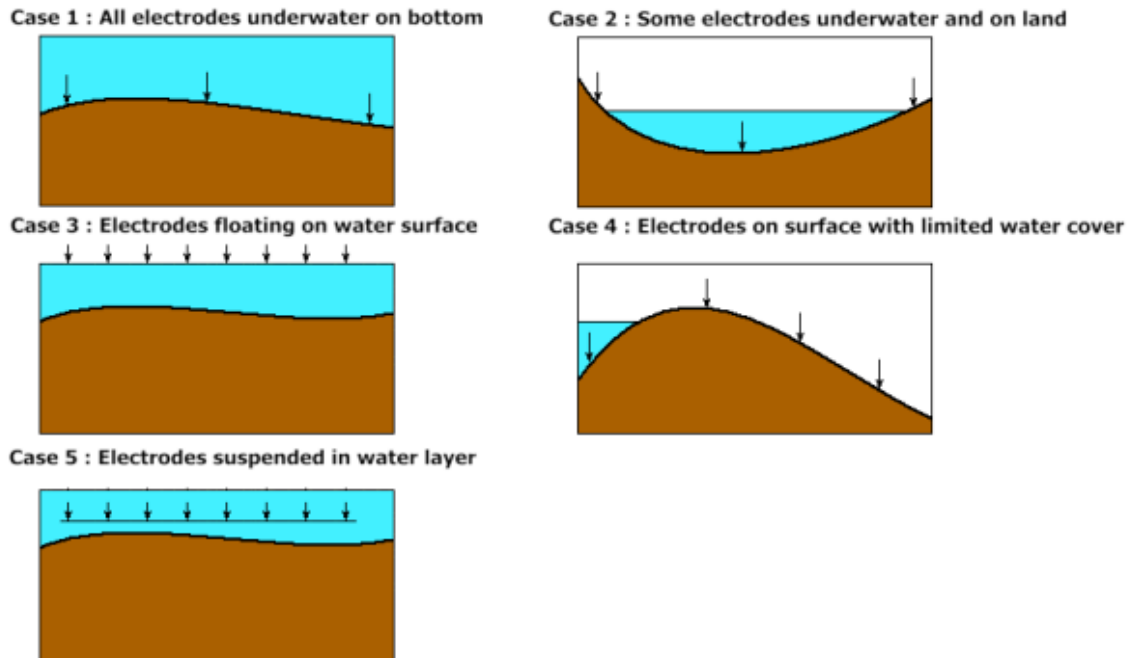
Figure 16. Five possible situations for aquatic surveys.
