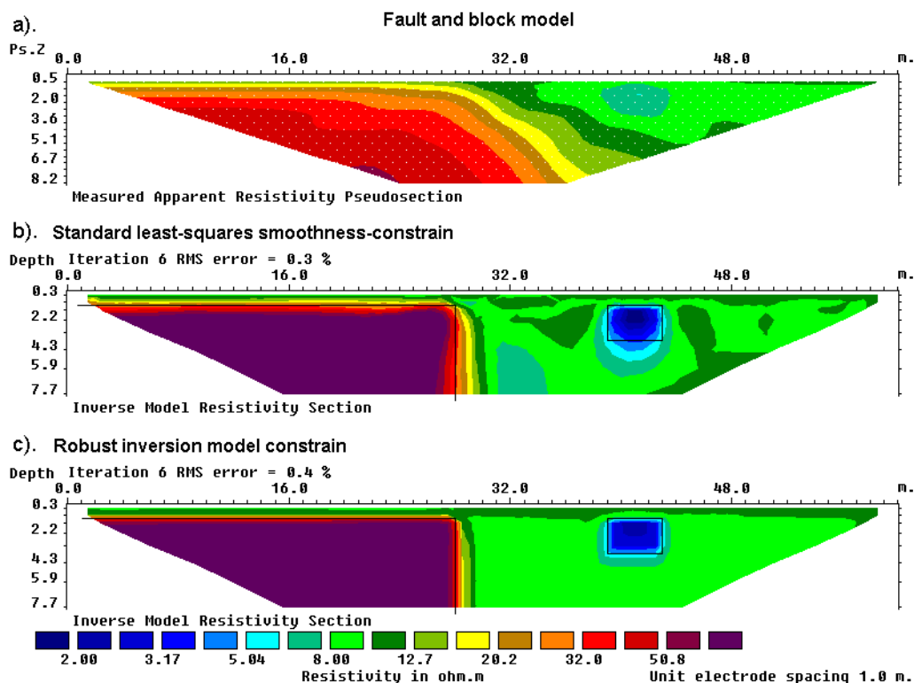
Figure 29. Example of inversion results using the smooth and robust inversion model constraint. (a) Apparent resistivity pseudosection. The inversion models produced by (b) the conventional least-squares smoothness-constrained method and (c) the robust or blocky inversion method.
