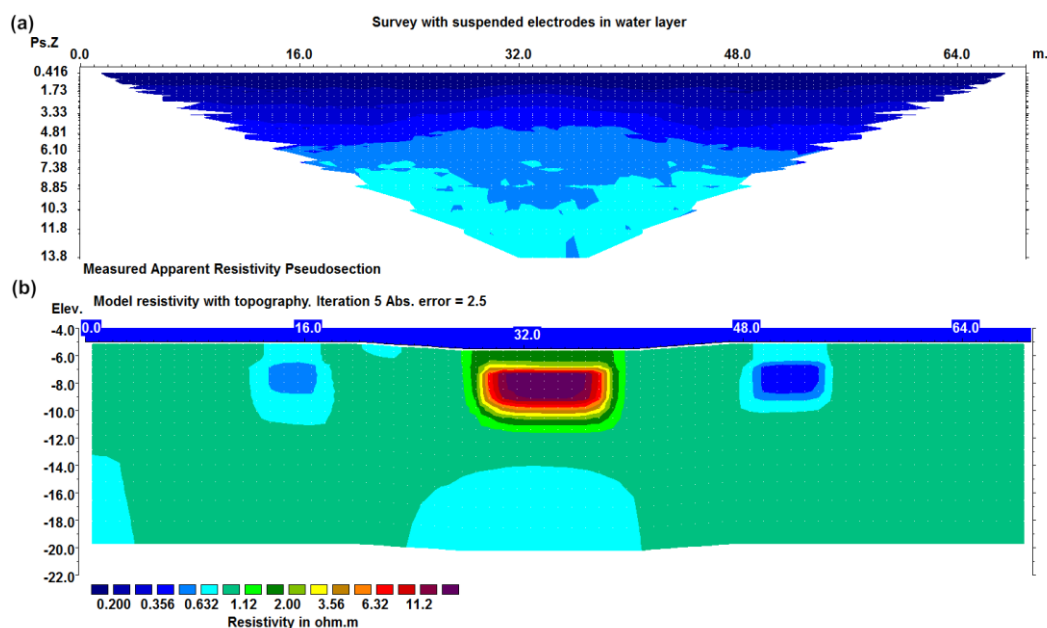
Figure 48. Example data set and inversion model for a survey with a streamer suspended in a water layer. (a) Apparent resistivity pseudosection and (b) inversion model section.
