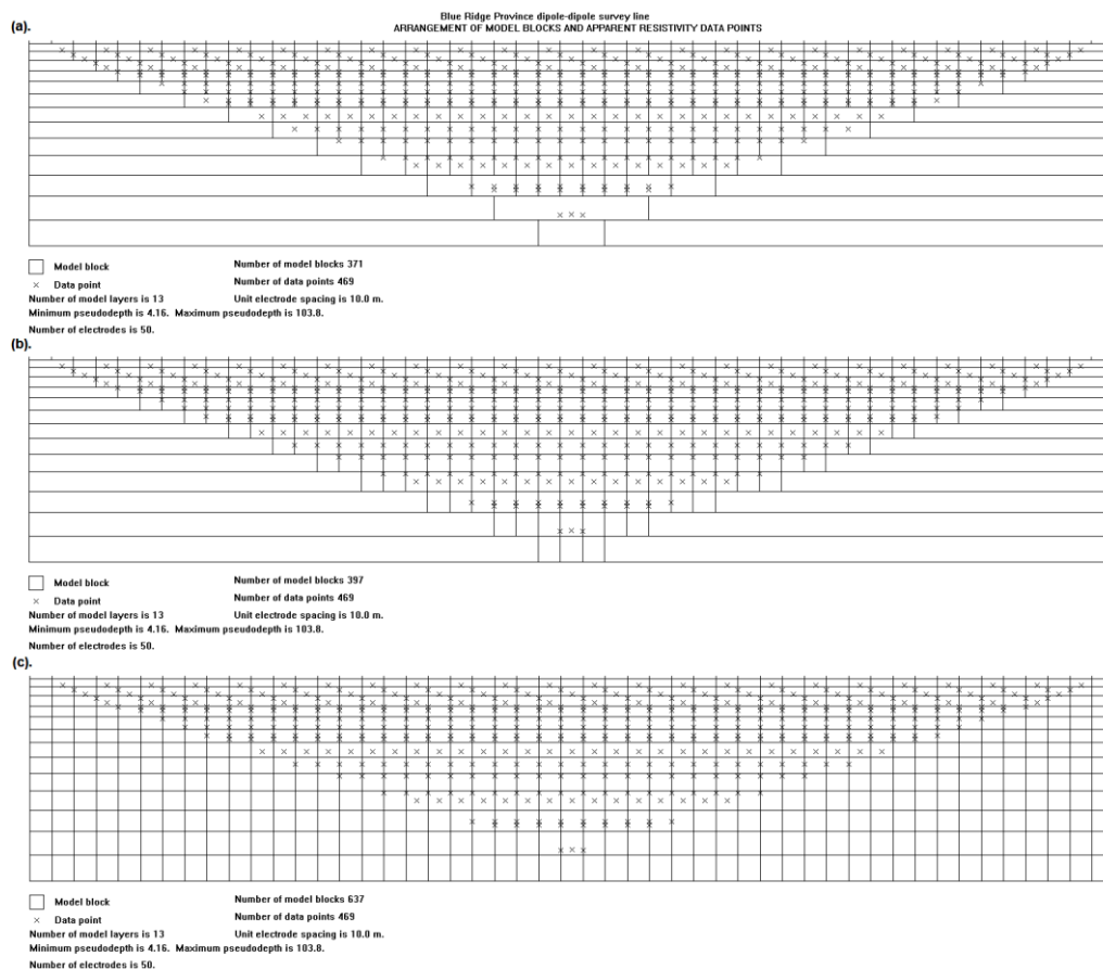
Figure 33. Different possible arrangement of model blocks for the same data set. (a) Using wider blocks at sides and bottom, (b) blocks of equal width, (c) model blocks extended to ends of survey line.
