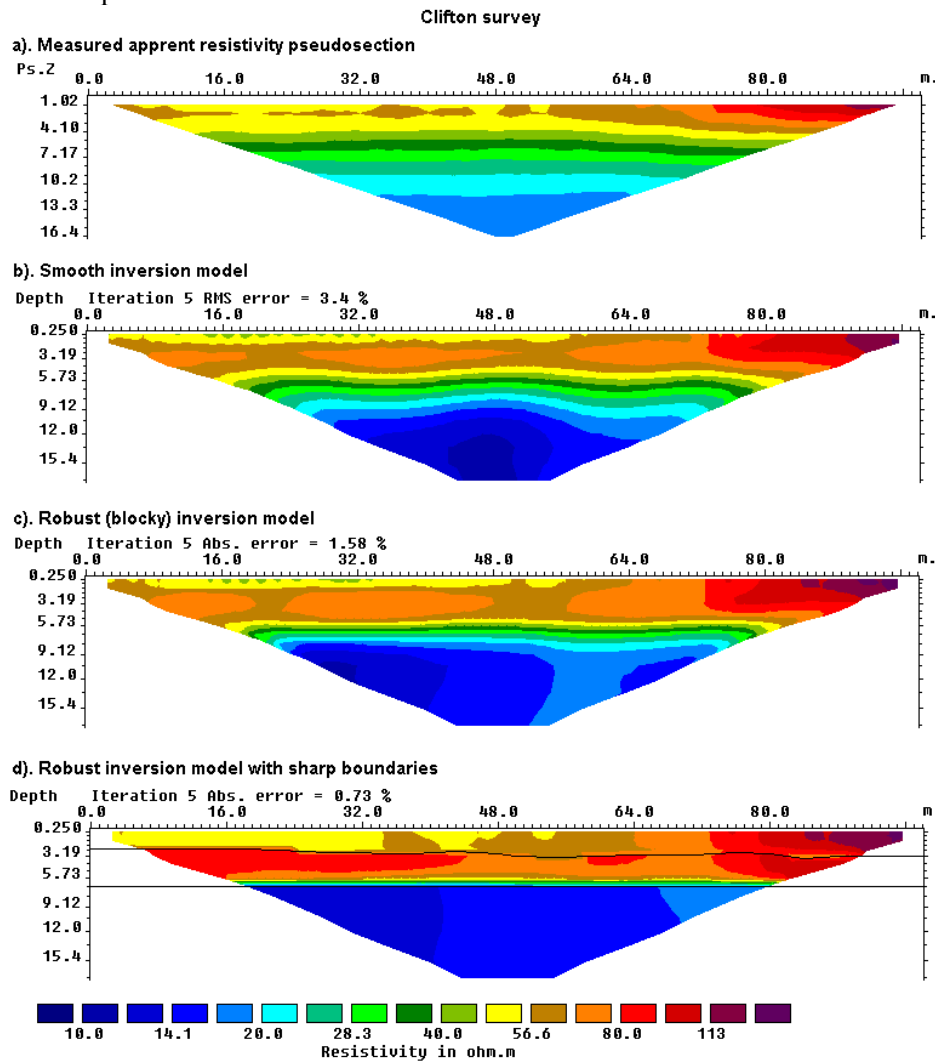
Figure 19. Models for the Clifton survey from the different inversion methods are shown together. Note the boundary between the high resistivity sand layer and the underlying low resistivity clay layer is much better resolved in the blocky and sharp boundary inversion methods.
