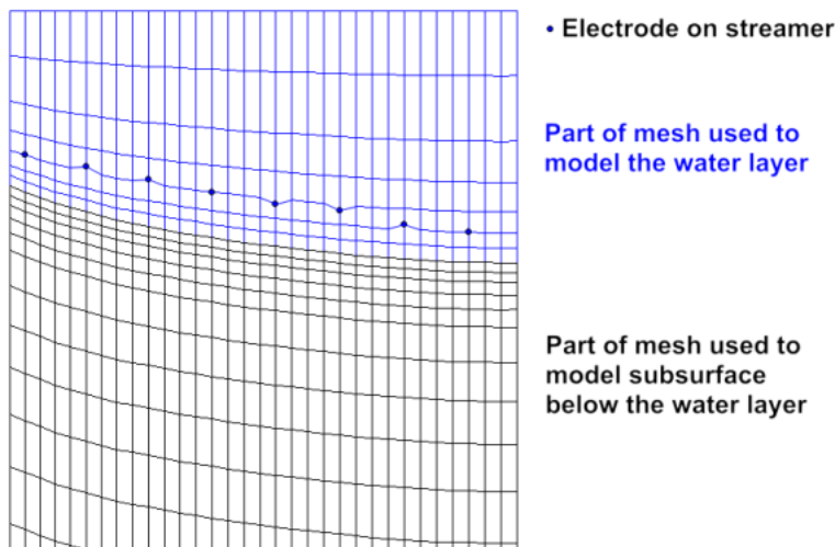
Figure 47. Mesh used to model water layer.
