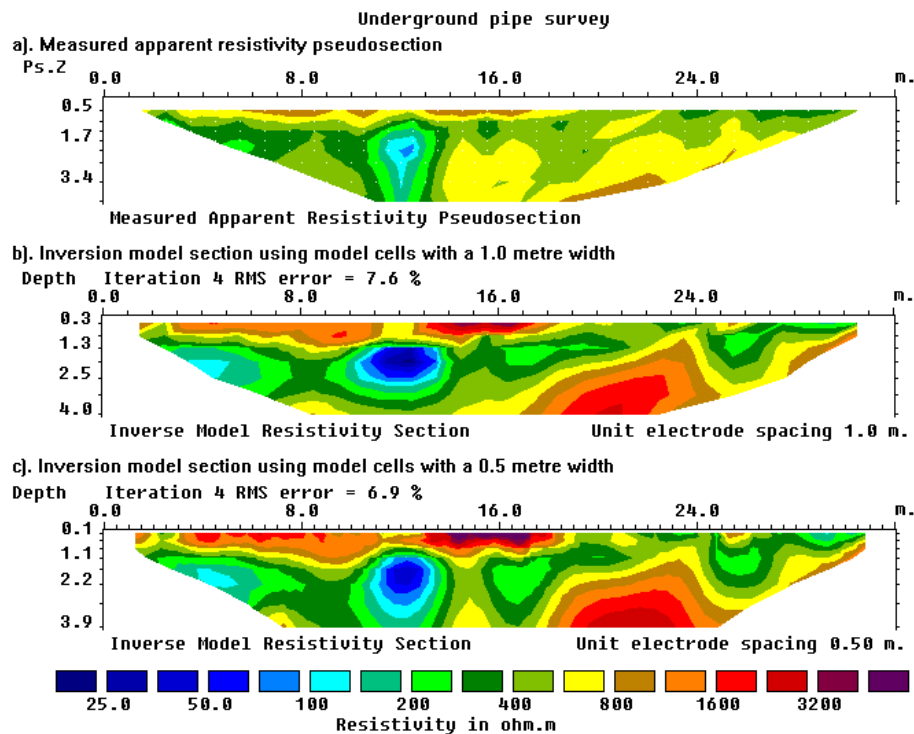
Figure 34. Example of inversion models using the standard and half-sized model blocks. (a) The apparent resistivity pseudosection for the PIPESCHL.DAT data set. The inversion models using (b) blocks with a width of 1.0 meter that is the same as the actual unit electrode, and (c) using narrower blocks with a width of 0.5 meter.
