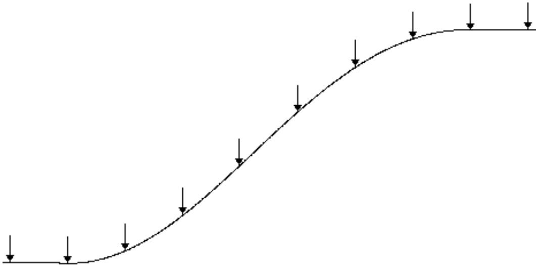
Figure 8. Arrangement of the electrodes along a survey line such that the true horizontal distance between adjacent electrodes is constant regardless of the slope of the ground surface. Note that the distance between adjacent electrodes along the ground surface is greater at the steeper part of the slope.
