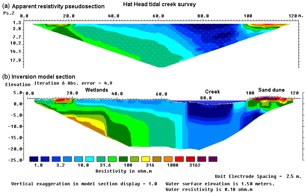
Figure 17. Hat Head land and underwater survey. (a) Apparent resistivity pseudosection (Wenner array) from the Hat Head tidal creek survey and (b) the inversion model. Note the creek between the 65 and 95 meters marks where the electrodes are underwater.
