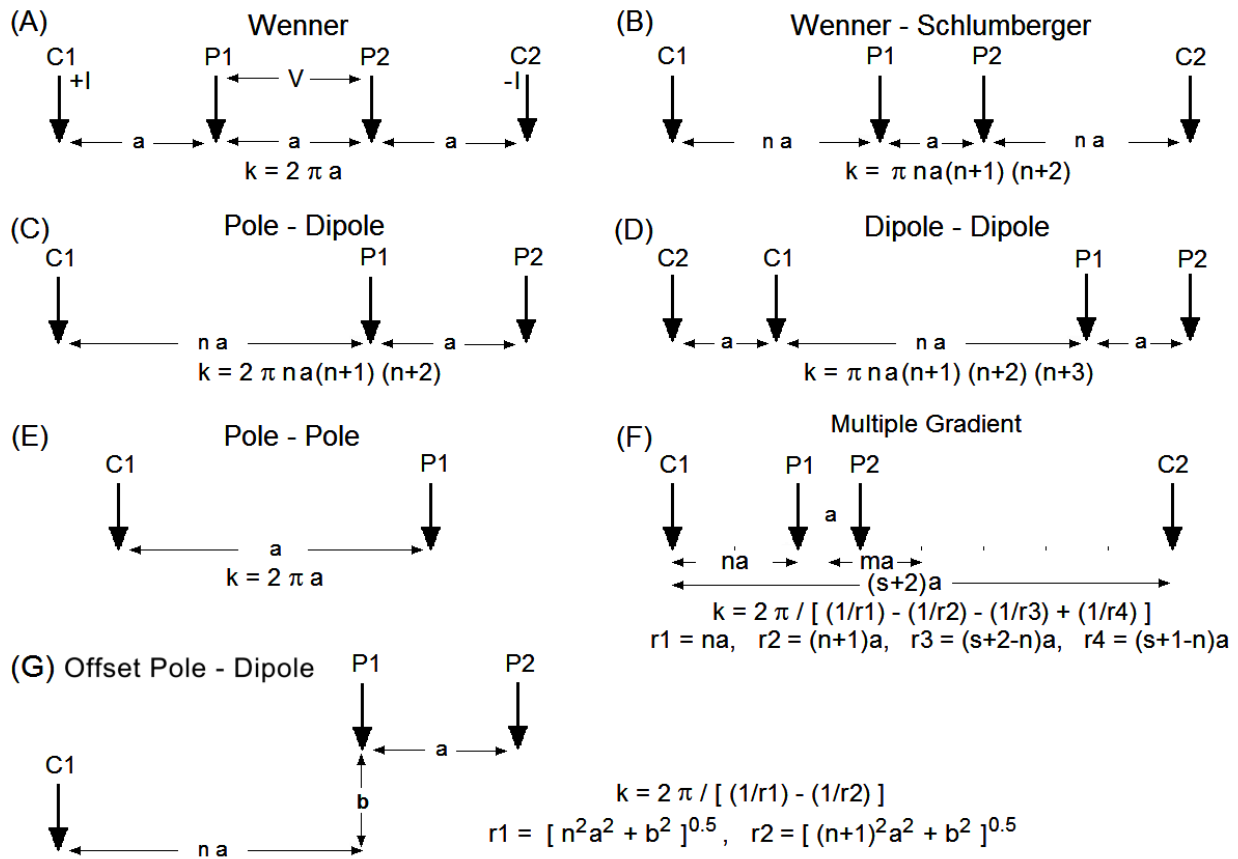
Figure 44. Arrangement of the electrodes for some commonly used arrays and their geometric factors.
