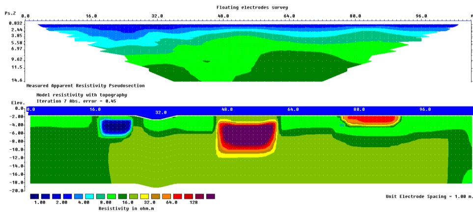
Figure 30. Example of inversion model with a fixed water layer. The inversion results of the WATER_FLOAT.DAT data is shown where the resistivity water layer (represented by the top blue layer in the model section) is fixed and model extends from below the water bottom.
