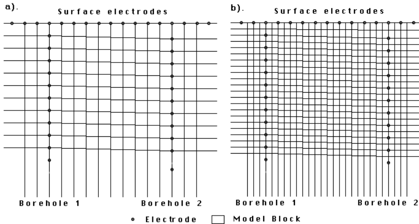
Figure 11. Arrangement of the electrodes in a cross-borehole survey. (a) The default standard model where the dimensions of the model blocks are equal to the spacing between the electrodes. (b) An alternative model with finer blocks with dimensions about half the spacing between the electrodes.
