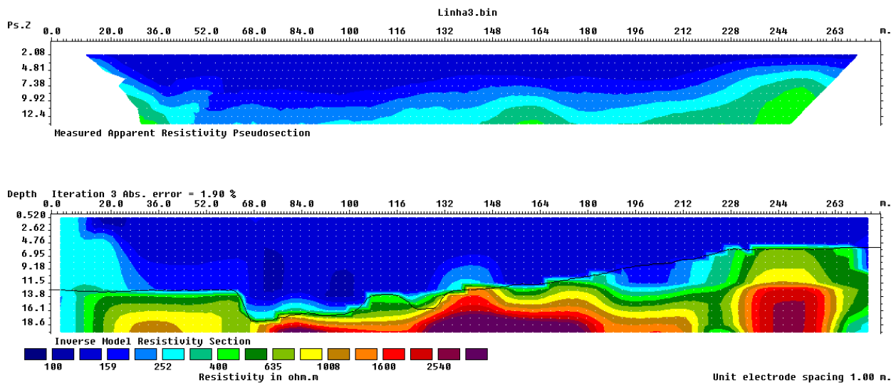
Figure 32. Inversion model for the survey with floating electrodes along the along the São Francisco River in Brazil. The thin black line indicates the water bottom boundary.
