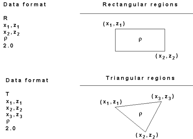
Figure 15. Fixing the resistivity of rectangular and triangular regions of the inversion model.
