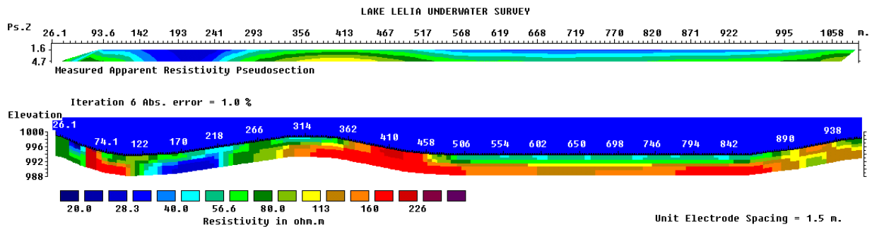
Figure 18. Lake Lelia underwater survey apparent resistivity pseudosection and model resistivity section. Courtesy of Technos Inc., USA.
