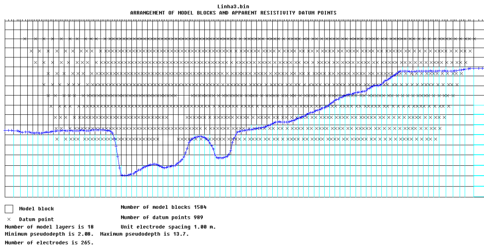
Figure 31. Arrangement of model blocks and the water bottom boundary for an arrangement with the water layer incorporated into the inversion model.
