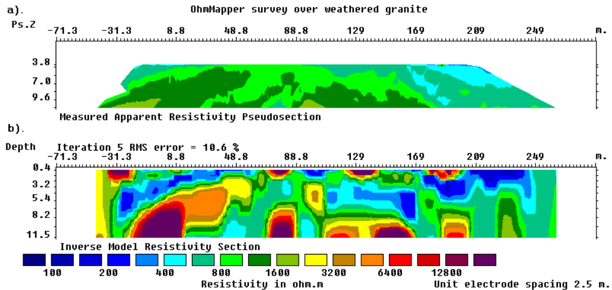
Figure 46. Example OhmMapper data set and inversion model. (a) Apparent resistivity pseudosection measured with an OhmMapper mobile resistivity surveying system. (b) Model section obtained by RES2DINV program.
