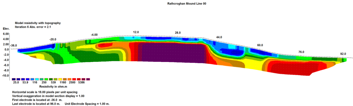
Figure 49. Example display with topography for the RATCHRO.INV file.
