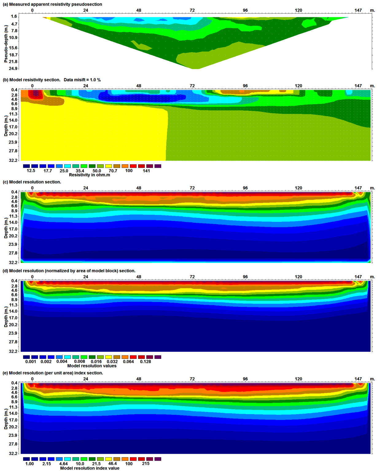
Figure 39. Model resolution sections for the LANDFIL.DAT data set. (a) Apparent resistivity pseudosection. (b) Inversion model section. (c) Model resolution section. (d) The model resolution normalized by the cross-section area of the model block. (e) The model resolution index (after normalization by model block area) section.
