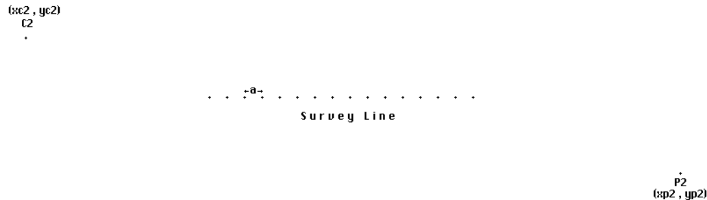
Figure 10. A schematic diagram of the arrangement of the electrodes along the survey line in a pole-pole survey with positions of the C2 and P2 electrodes specified.
