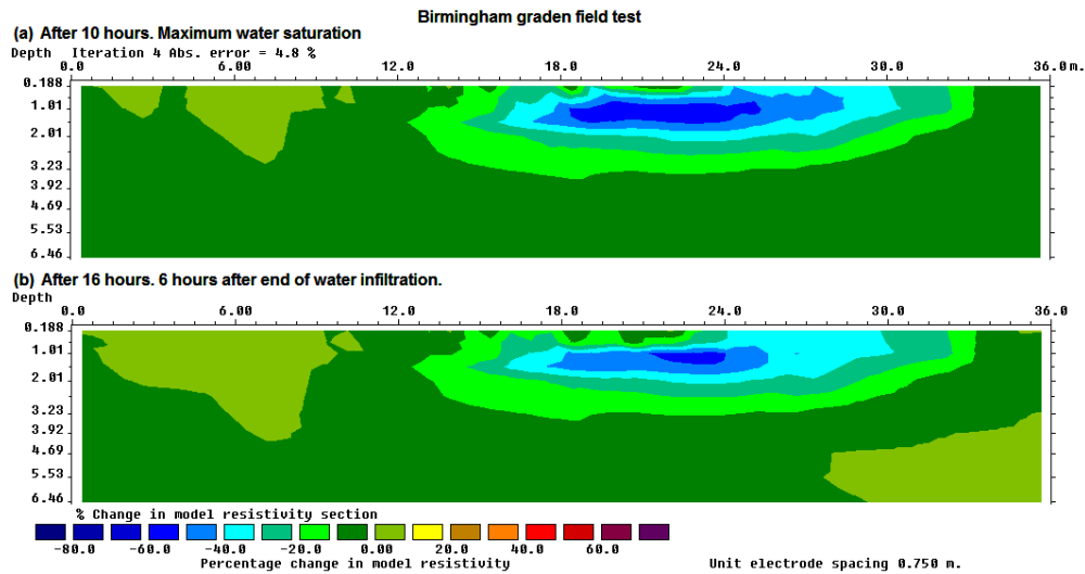
Figure 41. Sections showing the change in the subsurface resistivity values with time obtained from the inversion of the data sets collected during the infiltration and recovery phases of the study.
