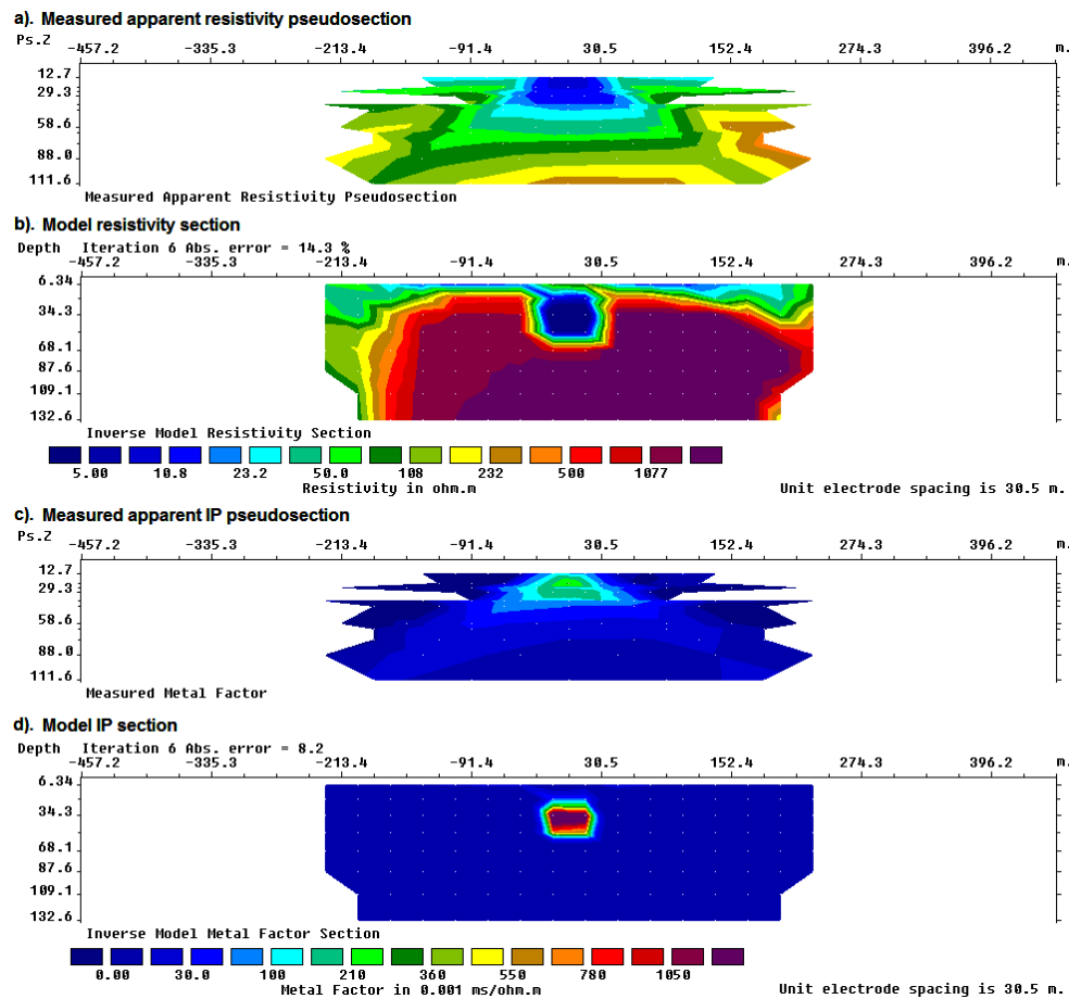
Figure 14. Magusi River ore body resistivity and I.P. sections. (a) Apparent resistivity pseudosection, (b) resistivity model section, (c) apparent metal factor pseudosection and (d) metal factor model section.
