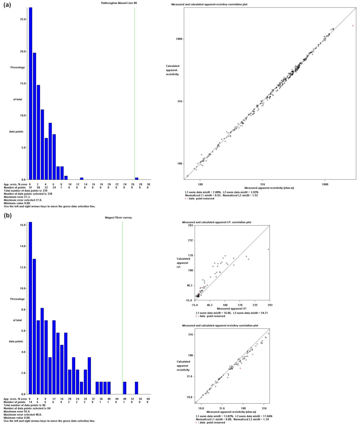
Figure 43. Histogram and scatter plots for the inversion results of the (a) RATHCRO.DAT and (b) IPMAGUSI.DAT data sets.
