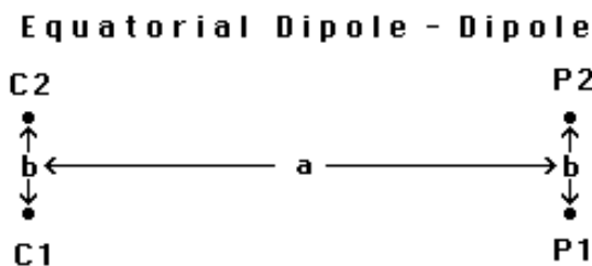
Figure 4. Arrangement of electrodes for the equatorial dipole-dipole array.
