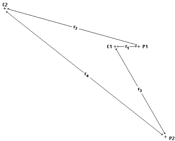
Figure 9. A schematic diagram of the arrangement of the electrodes in an actual field pole-pole measurement.
