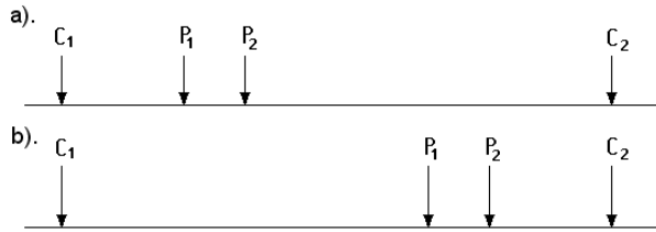
Figure 26. Two different configurations of the gradient array with the same pseudodepth but with the potential electrodes at different sides of the array. Gradient array configuration with (a) right parity and (b) left parity.
