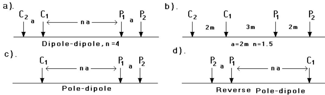
Figure 5. Arrangement of the electrodes for the dipole-dipole and pole-dipole arrays. (a) Dipole-dipole array with integer ' n ' factor. (b) Example of dipole-dipole array with non-integer " n " value. Arrangement of the electrodes for (c) the "forward" and (d) "reverse" pole-dipole arrays.
