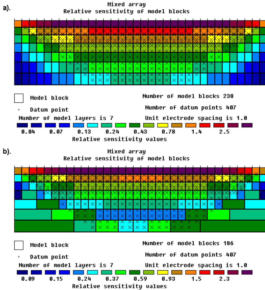
Figure 35. Two arrangements of model blocks using the extended model and sensitivity values methods. The arrangement of the model blocks used by the program for the inversion of the MIXEDWS.DAT data set using (a) the default extended model and (b) a model generated so that any single block the does not have a relative sensitivity value that is too small.
