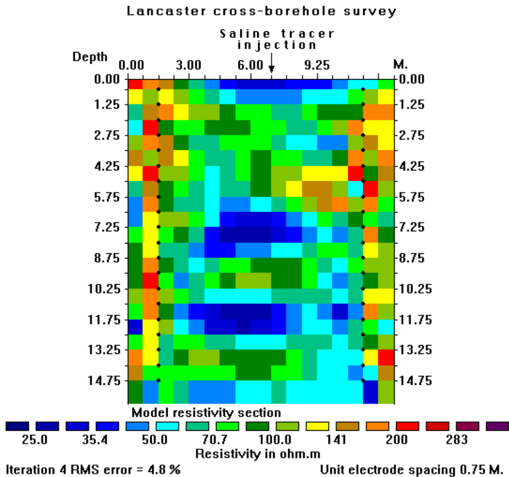
Figure 13. Model obtained from the inversion of data from a cross-borehole survey to map the flow of a saline tracer. Note the low resistivity zones near the surface (where the tracer was injected) and below a depth of 7 meters. The locations of the borehole electrodes are shown by small black dots.
